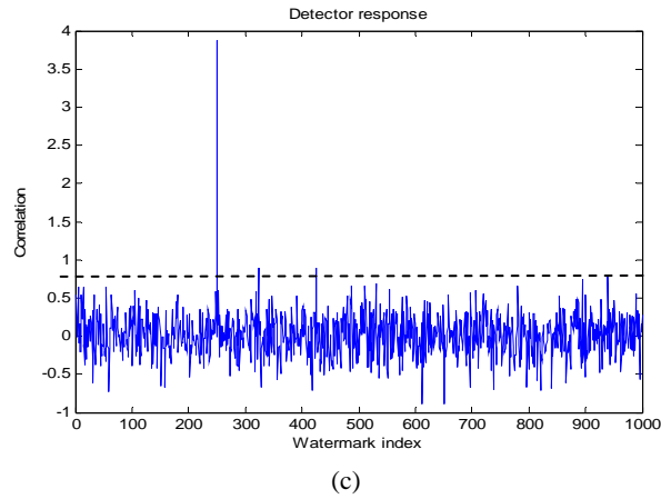
Fig. 5. (a) Original image. (b) Watermarked image. (c) Detection threshold experimentally. T is set to be 0.75.
